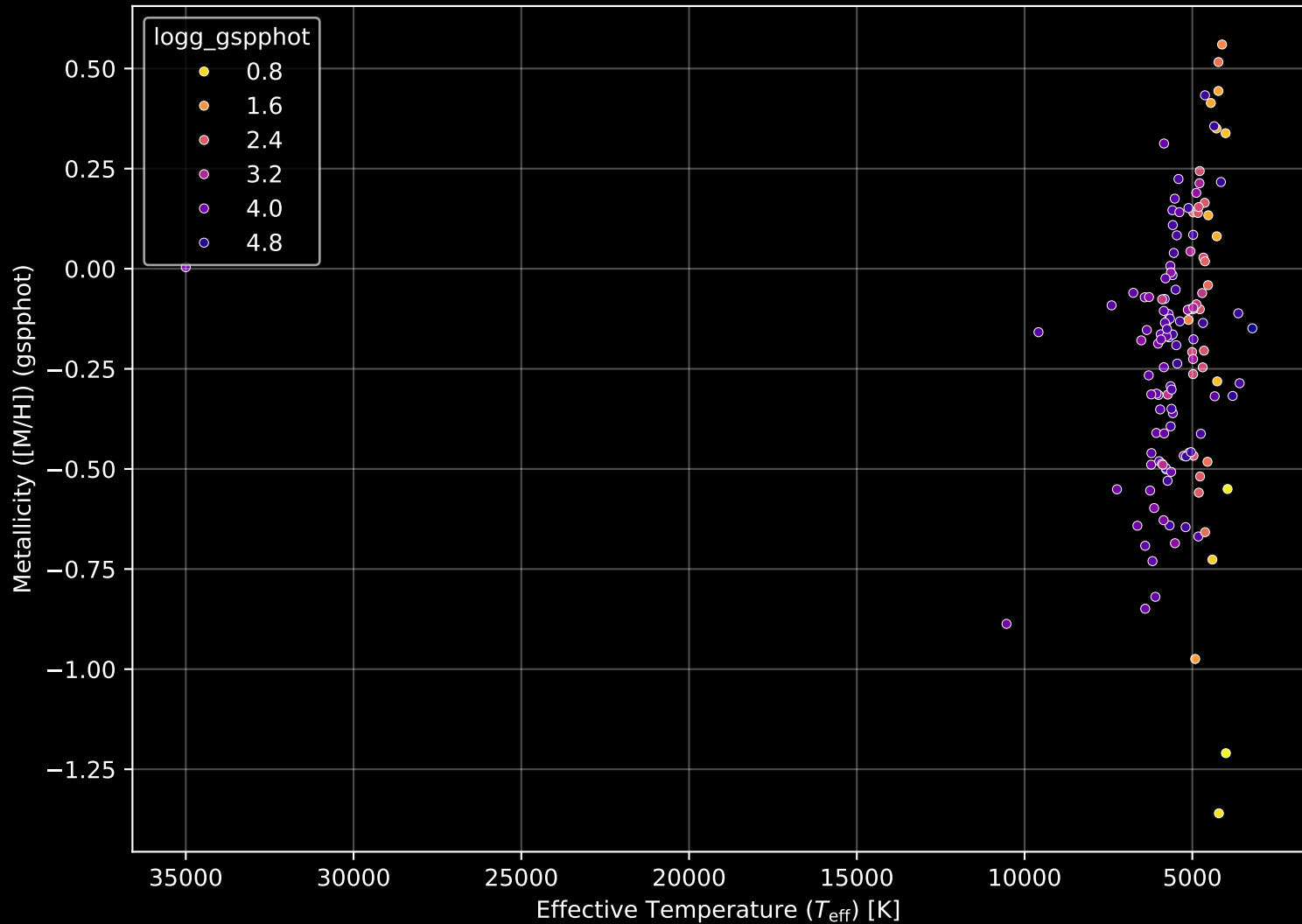
APOGEE DR17 Field: [276-30-O_TESS] Stellar Population Parameters (n= 136)
