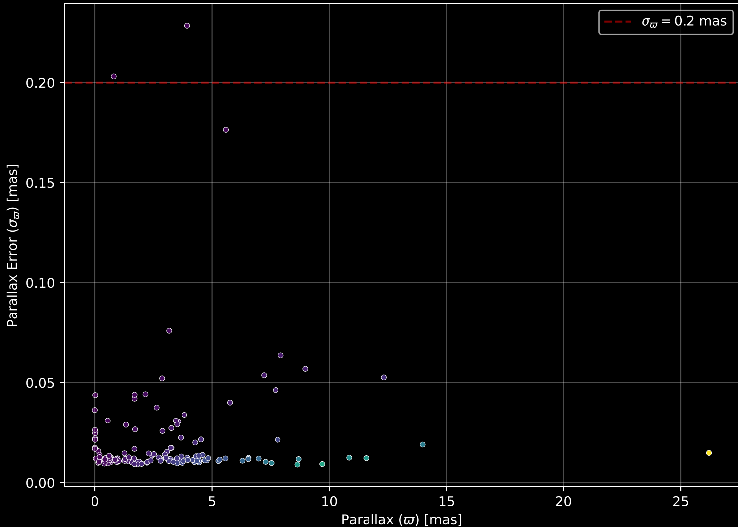
APOGEE DR17 Field: [276-30-O_TESS] Parallax Quality (n= 136)
