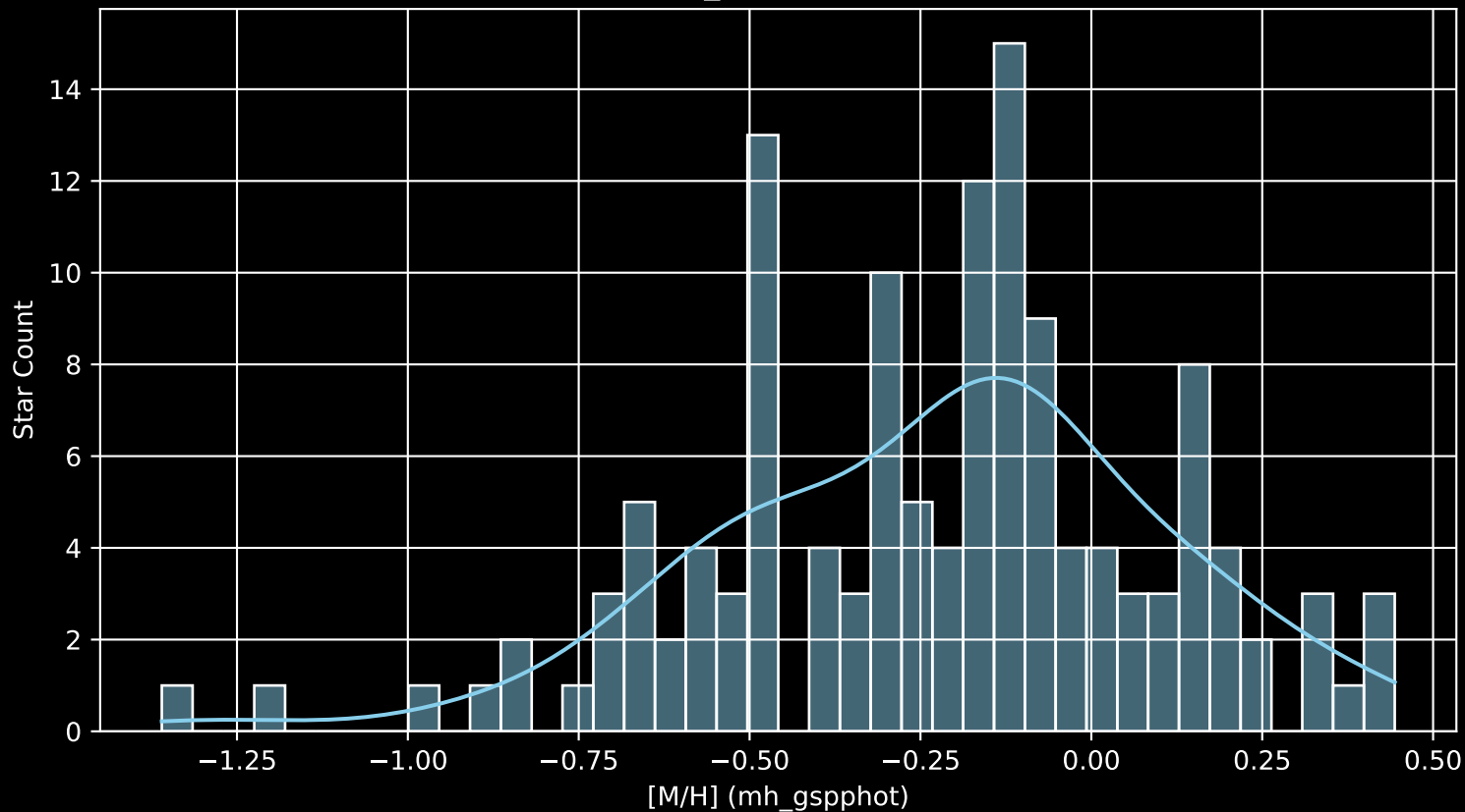
APOGEE DR17 Field: [276-30-O_TESS [M/H] (mh_gspphot) (n= 134)
