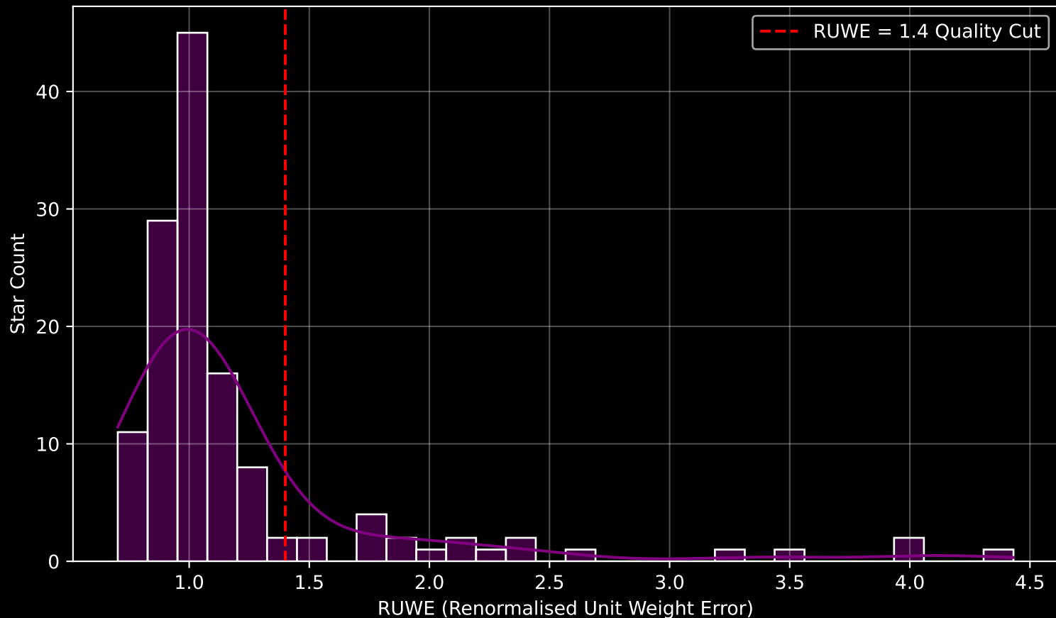
GAPOGEE DR17 Field [276-30-O_TESS] RUWE Distribution (n= 131)
