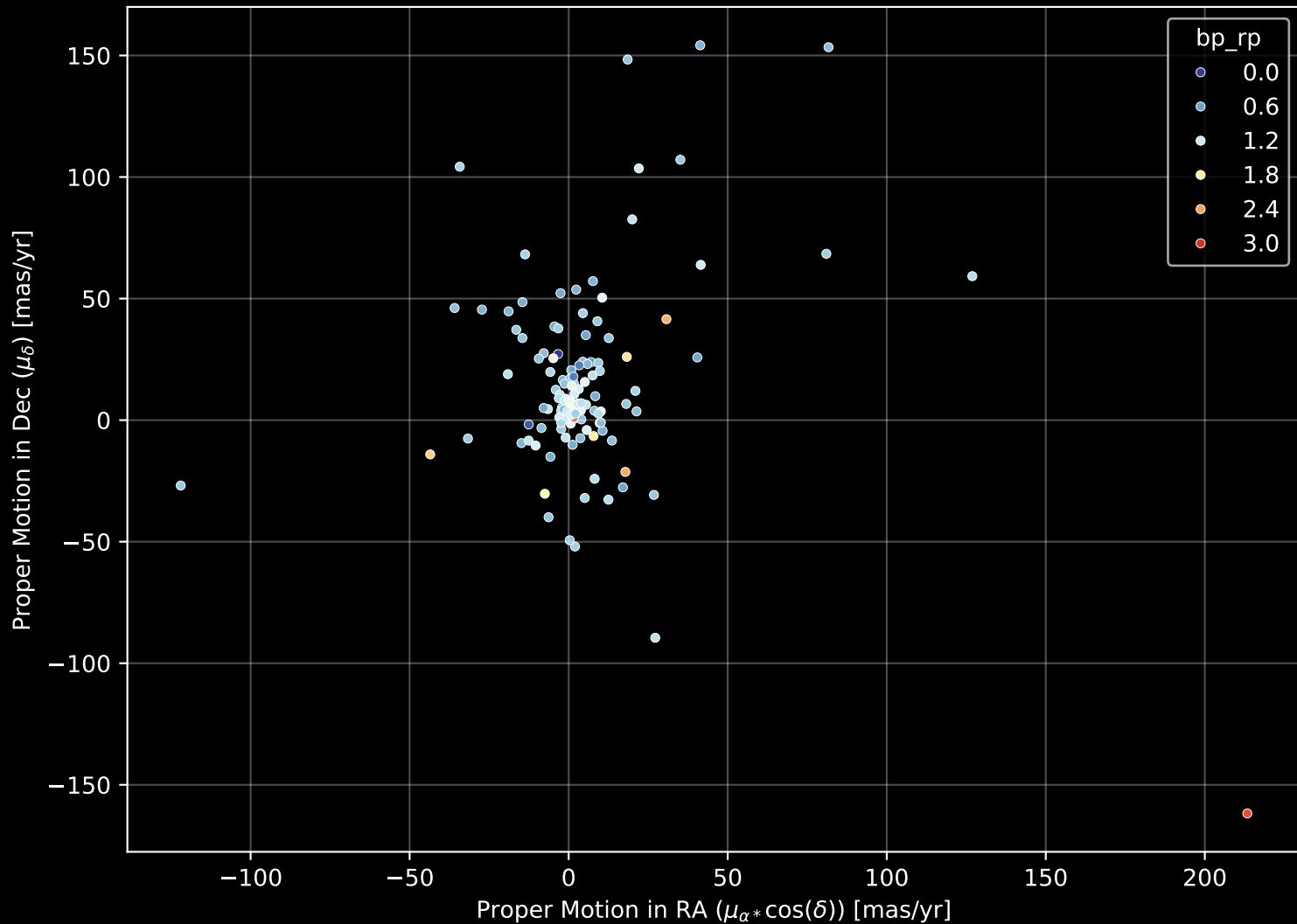
APOGEE DR17 Field: [276-30-O_TESS] Proper Motion Diagram (n= 136)
