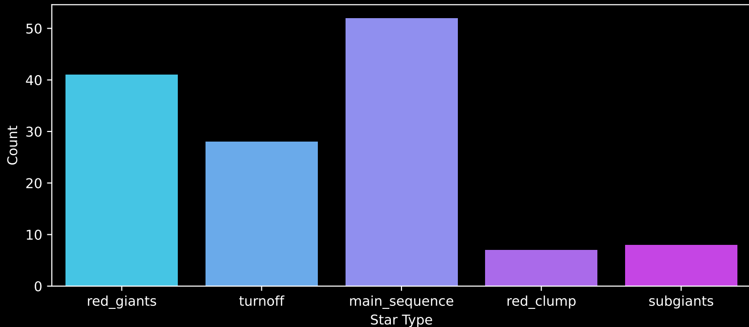
APOGEE DR17 Field: [276-30-O_TESS] Count plot of Star Type
